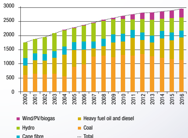
CHANGES IN ELECTRICITY PRODUCTION by energy type
